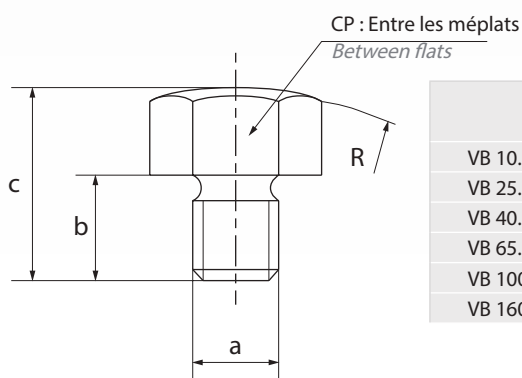
Vis de pression à tête bombée Pressure screw with mushroom head
