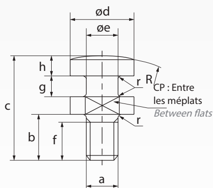
Vis de pression à tête bombée Pressure screw with mushroom head
